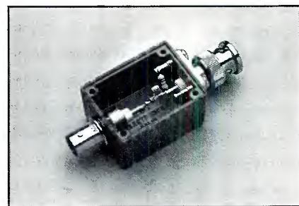
Figure 4. A small metal box such as this provides a convenient and shielded environment for the attenuator circuits.
